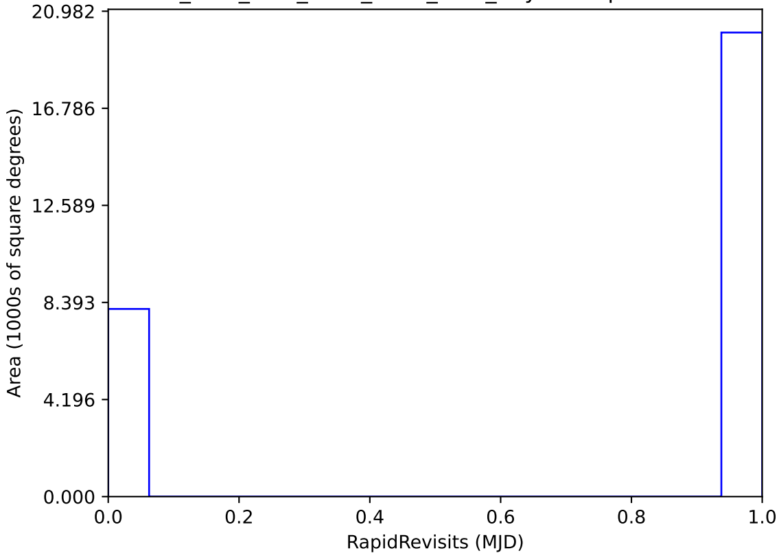
ddf_acor_sf10_ls40_lsr50_v3.4_10yrs : RapidRevisits
