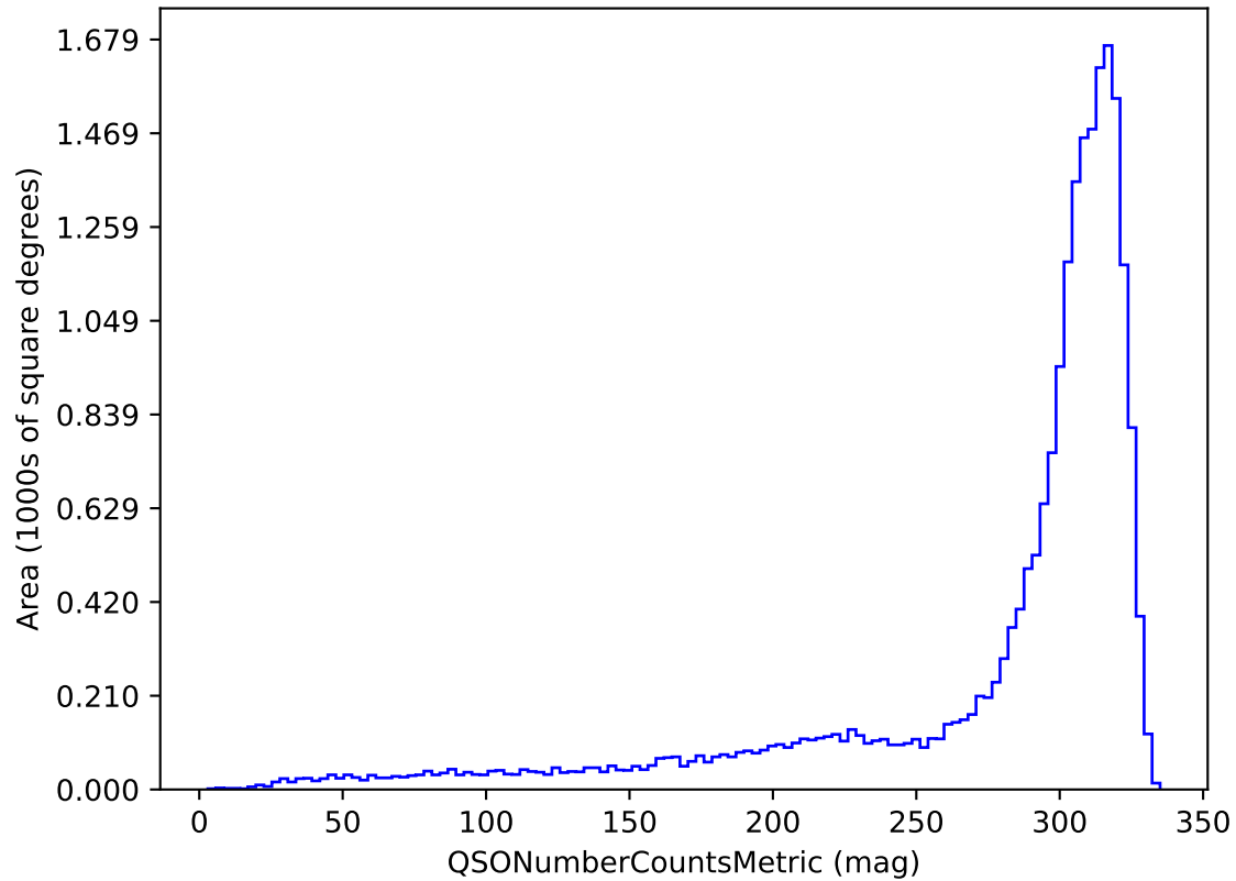
ddf_acor_sf10_lsf40_lsr50_v3.4_10yrs u band and non-DD: QSONumberCountsMetric
