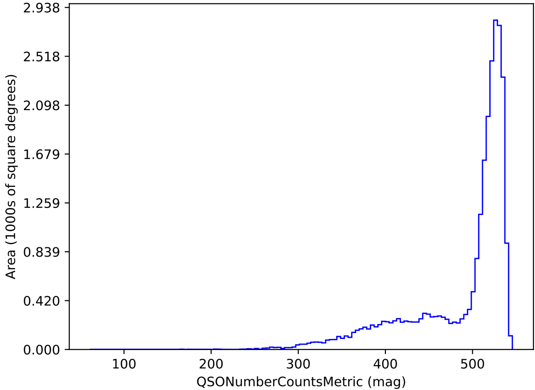
ddf_acor_sf10_lsf40_lsr50_v3.4_10yrs r band and non-DD: QSONumberCountsMetric
