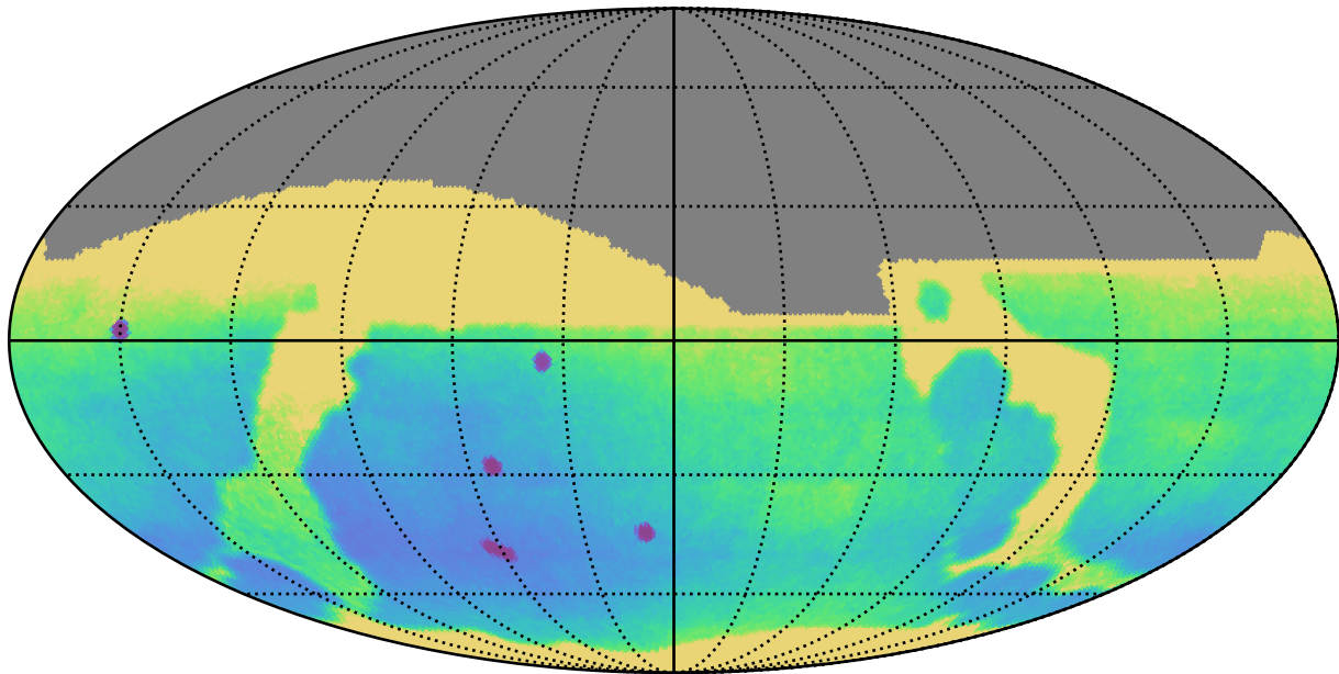
ddf_acor_sf10_lsf40_lsr50_v3.4_10yrs : Parallax Uncert @ 24.0
