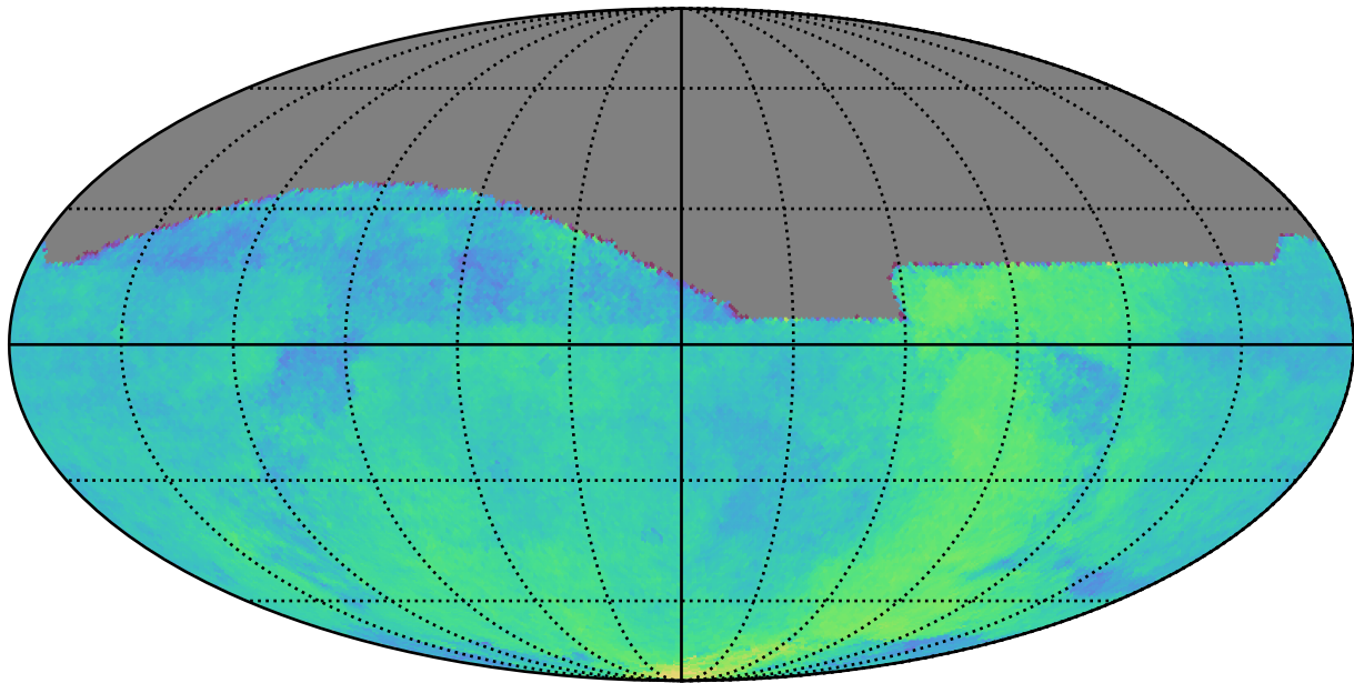
ddf_acor_sf10_lsf40_lsr50_v3.4_10yrs : Parallax Coverage @ 24.0
