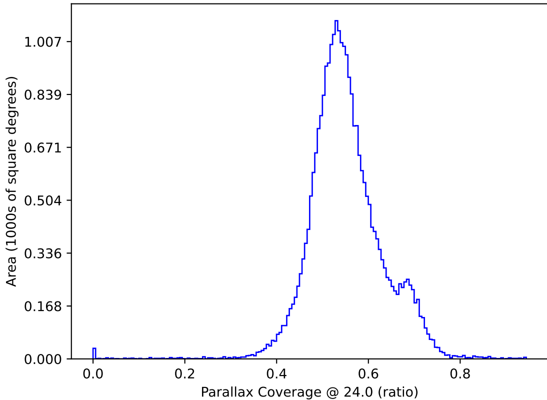
ddf_acor_sf10_lsf40_lsr50_v3.4_10yrs : Parallax Coverage @ 24.0
