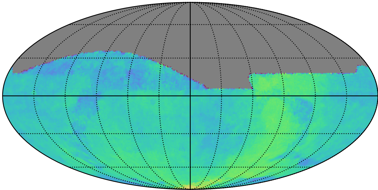
ddf_acor_sf10_lsf40_lsr50_v3.4_10yrs : Parallax Coverage @ 22.4
