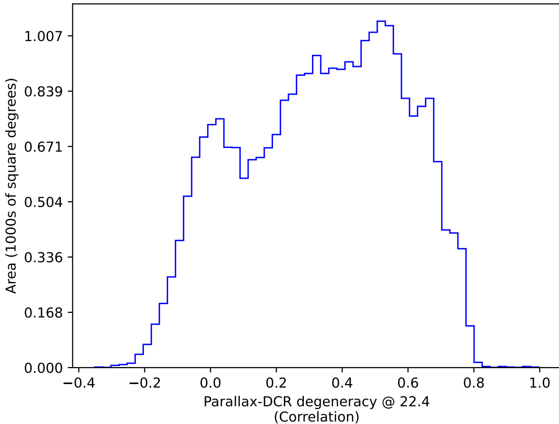
ddf_acor_sf10_ls40_lsr50_v3.4_10yrs : Parallax-DCR degeneracy @ 22.4
