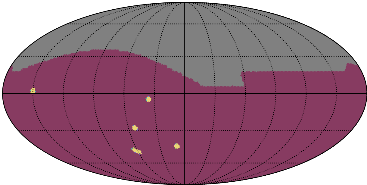
ddf_acor_sf10_lsf40_lsr50_v3.4_10yrs : NumberOfQuickRevisits
