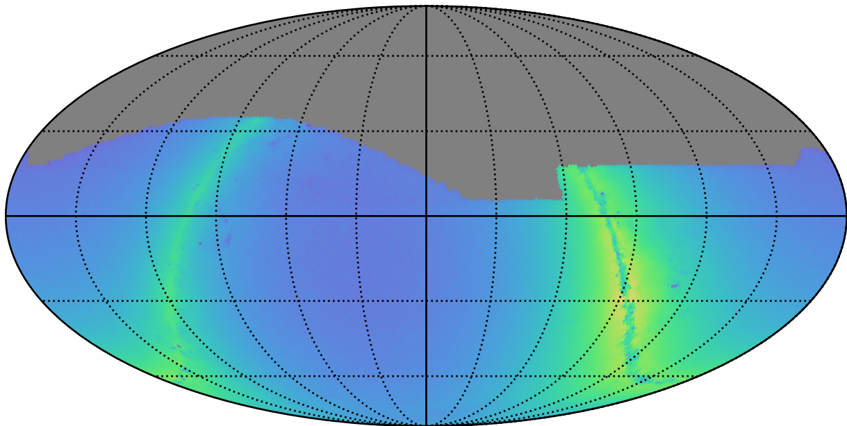
ddf_acor_sf10_lsf40_lsr50_v3.4_10yrs r: Nstars_no_crowding
