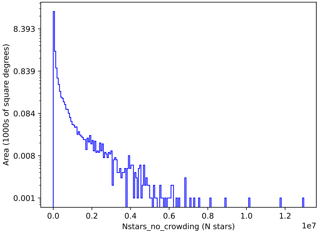
ddf_acor_sf10_ls40_lsr50_v3.4_10yrs g: Nstars_no_crowding
