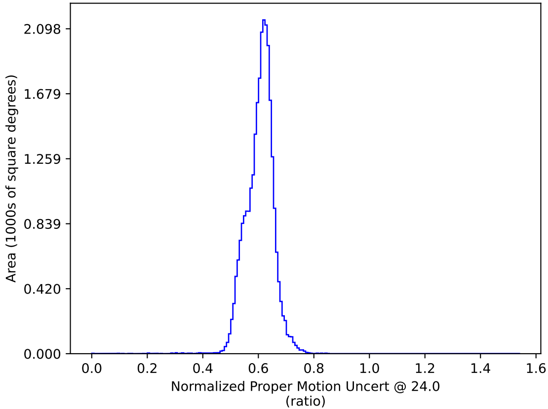
ddf_acor_sf10_lsf40_lsr50_v3.4_10yrs : Normalized Proper Motion Uncert @ 24.0
