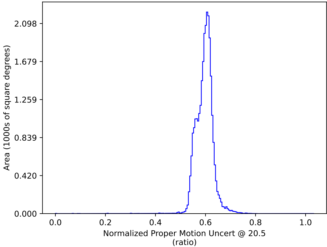
ddf_acor_sf10_lsf40_lsr50_v3.4_10yrs : Normalized Proper Motion Uncert @ 20.5
