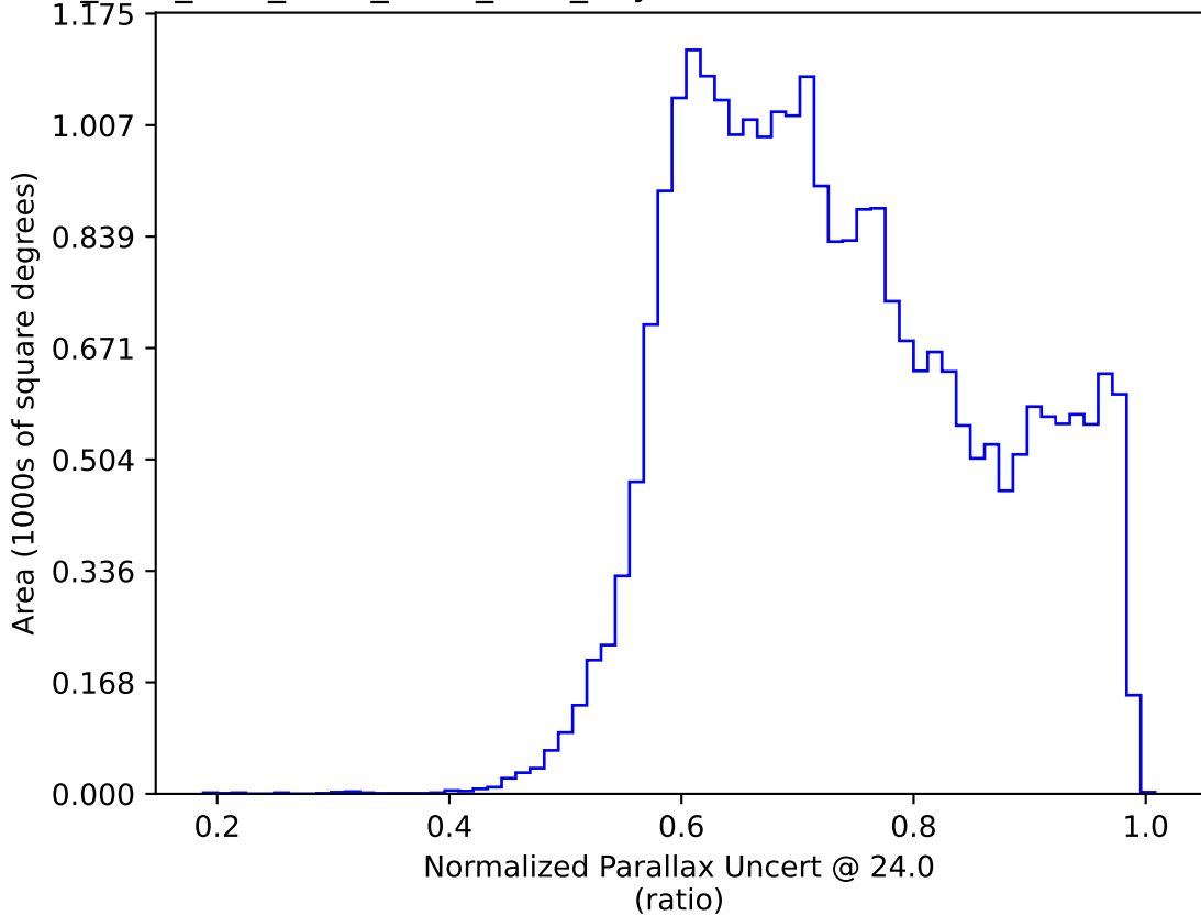
ddf_acor_sf10_lsf40_lsr50_v3.4_10yrs : Normalized Parallax Uncert @ 24.0
