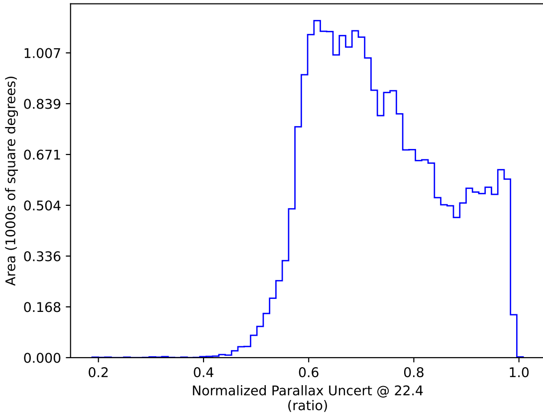
ddf_acor_sf10_lsf40_lsr50_v3.4_10yrs : Normalized Parallax Uncert @ 22.4
