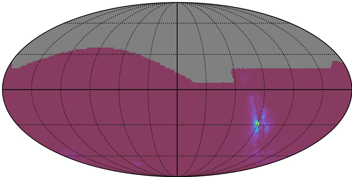
ddf_acor_sf10_lsf40_lsr50_v3.4_10yrs : NlcPoints
