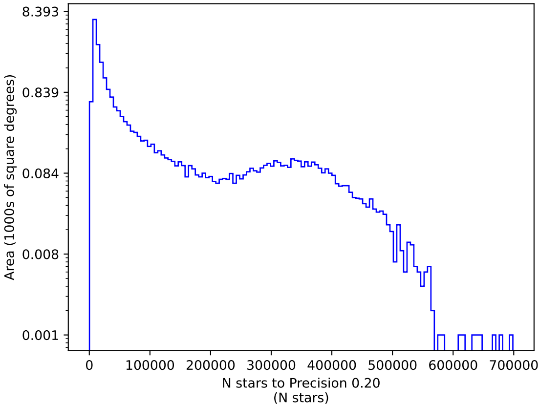
ddf_acor_sf10_lsf40_lsr50_v3.4_10yrs y: N stars to Precision 0.20
