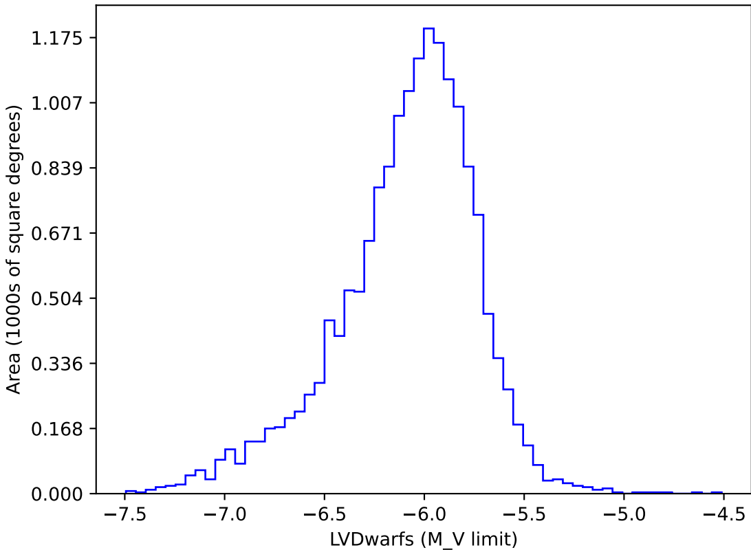
ddf_acor_sf10_lsf40_lsr50_v3.4_10yrs gi: LVDwarfs
