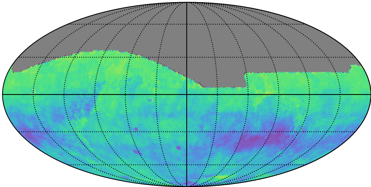
ddf_acor_sf10_lsf40_lsr50_v3.4_10yrs r: Kuiper rotSkyPos
