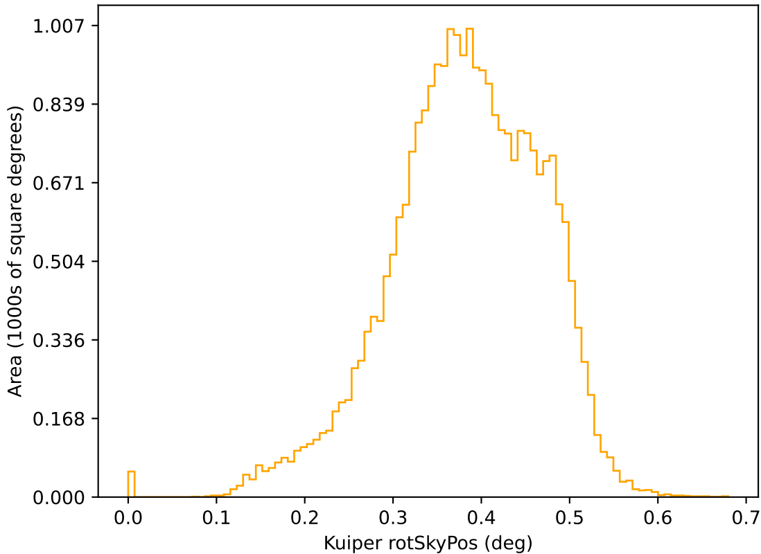
ddf_acor_sf10_lsf40_lsr50_v3.4_10yrs r: Kuiper rotSkyPos
