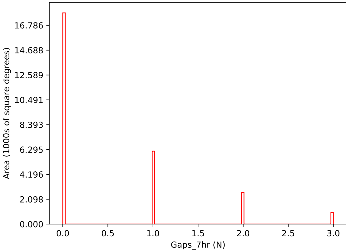
ddf_acor_sf10_lsf40_lsr50_v3.4_10yrs i band: Gaps_7hr
