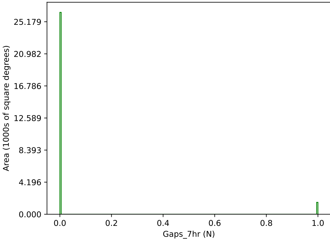
ddf_acor_sf10_lsf40_lsr50_v3.4_10yrs g band: Gaps_7hr
