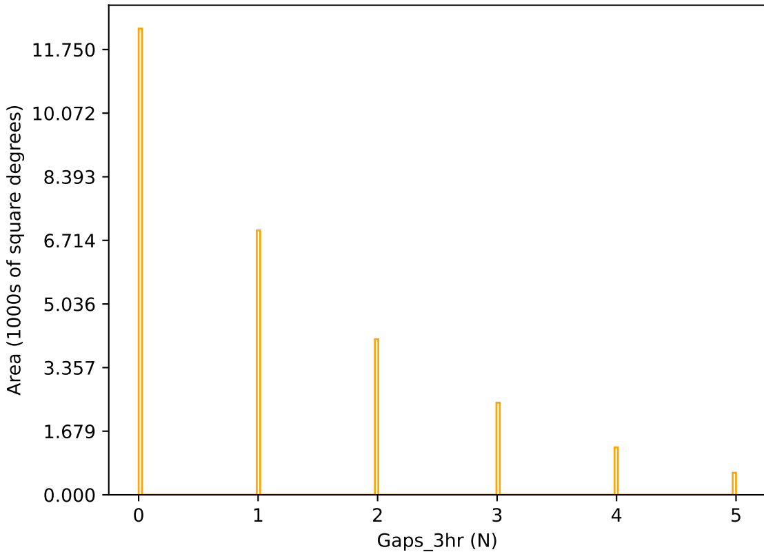
ddf_acor_sf10_lsf40_lsr50_v3.4_10yrs r band: Gaps_3hr
