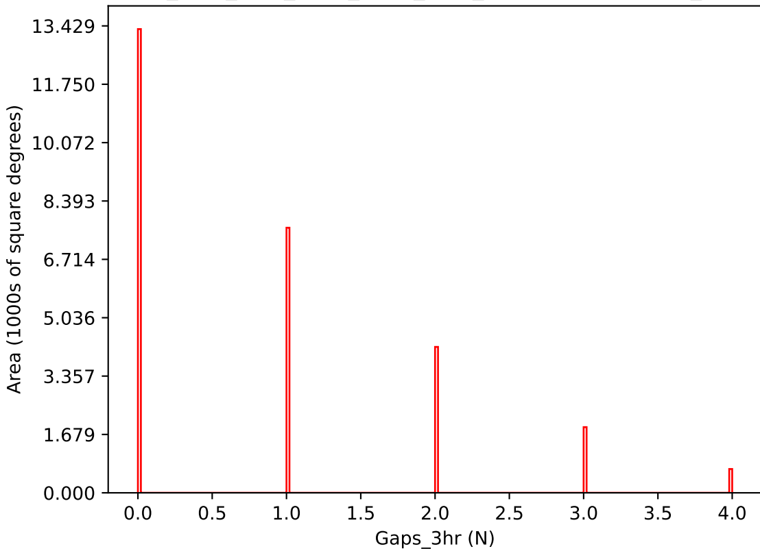
ddf_acor_sf10_lsf40_lsr50_v3.4_10yrs i band: Gaps_3hr
