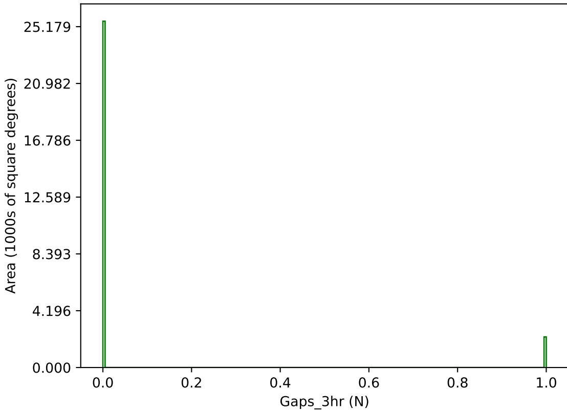
ddf_acor_sf10_ls40_lsr50_v3.4_10yrs g band: Gaps_3hr
