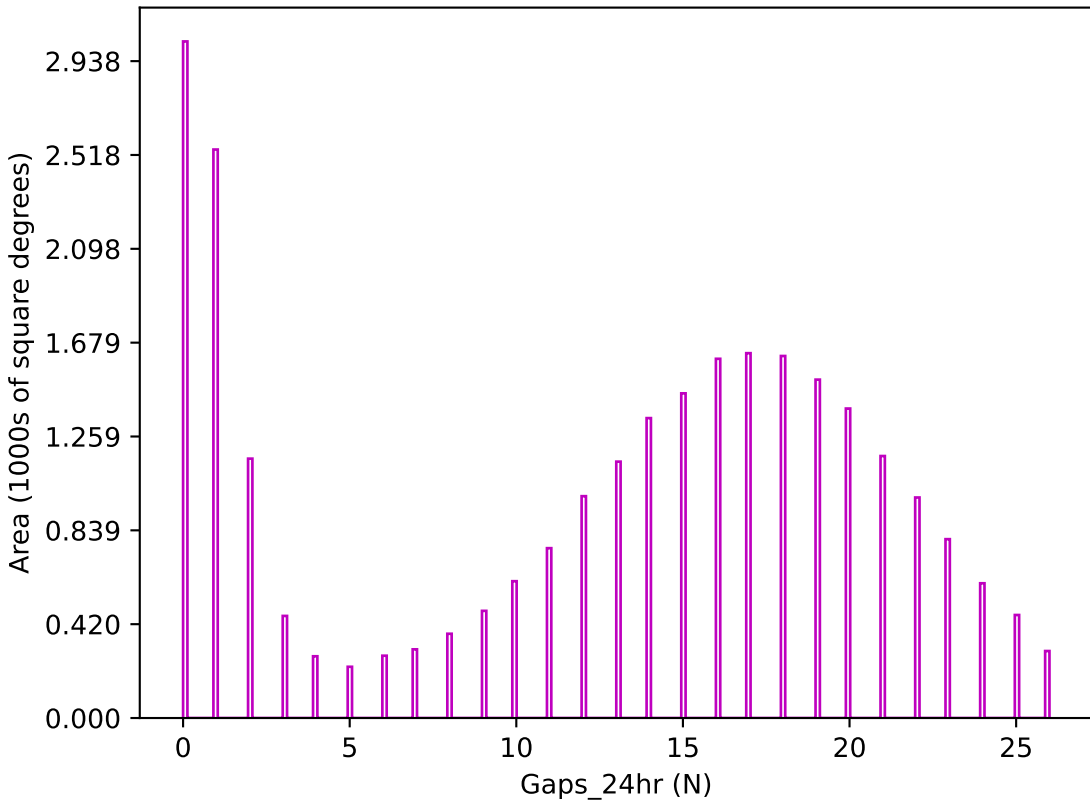
ddf_acor_sf10_ls40_lsr50_v3.4_10yrs z band: Gaps_24hr
