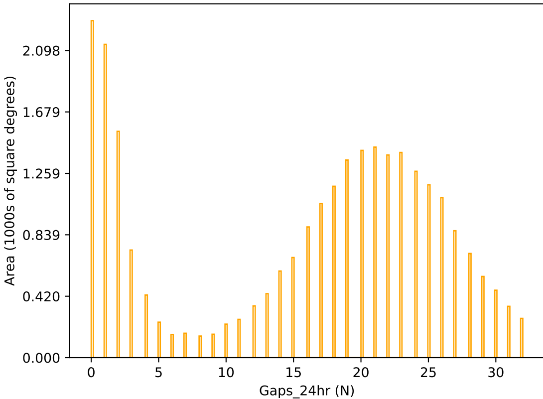
ddf_acor_sf10_ls40_lsr50_v3.4_10yrs r band: Gaps_24hr
