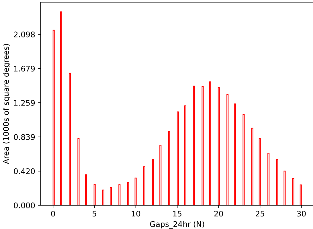
ddf_acor_sf10_lsf40_lsr50_v3.4_10yrs i band: Gaps_24hr
