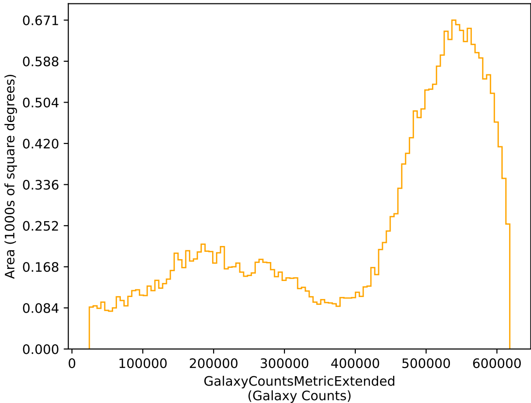
ddf_acor_sf10_lsf40_lsr50_v3.4_10yrs r: GalaxyCountsMetricExtended
