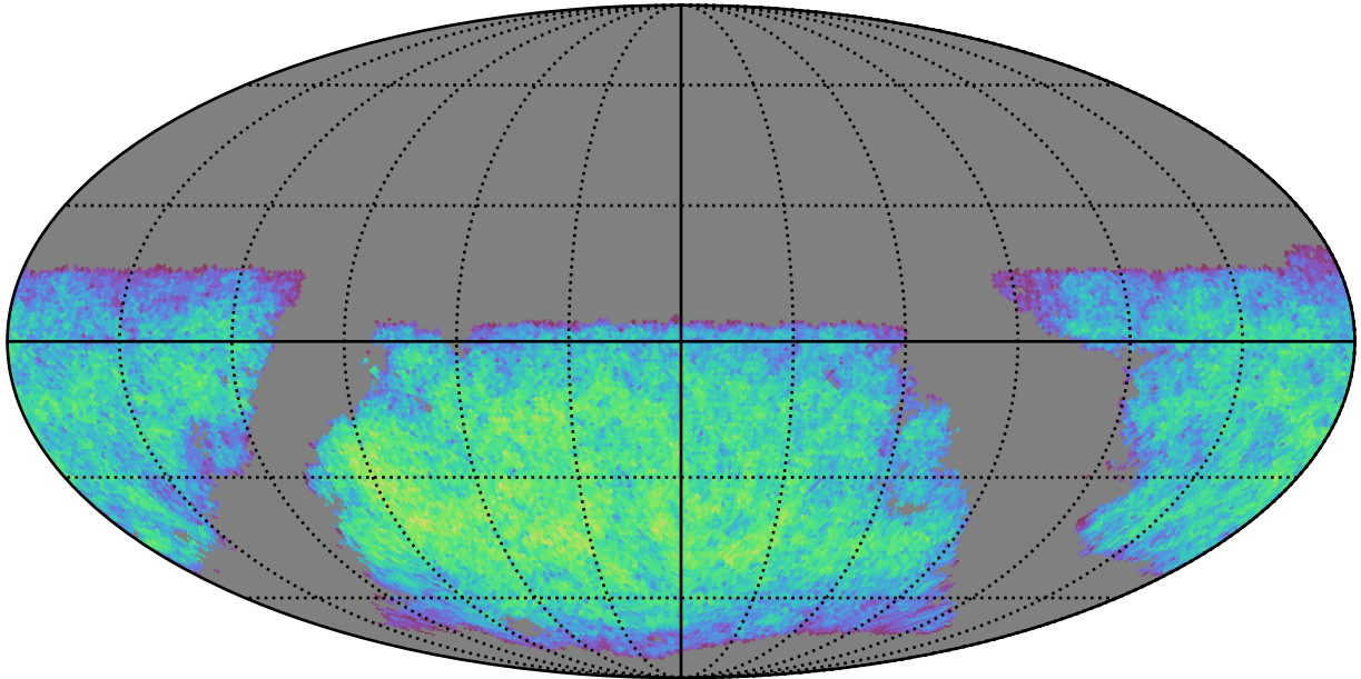
ddf_acor_sf10_lsf40_lsr50_v3.4_10yrs i band non-DD year 1: ExgalM5WithCuts
