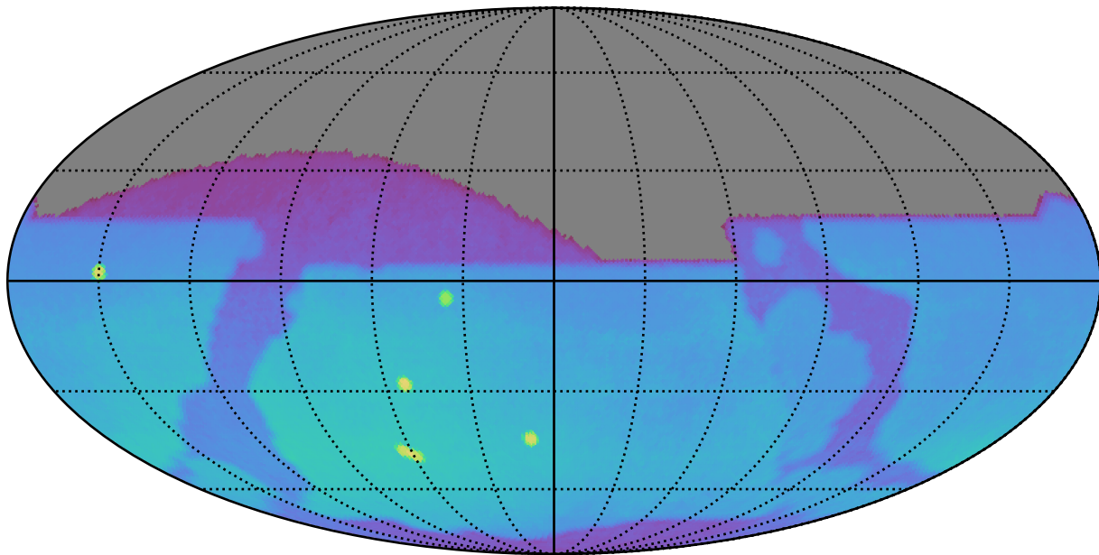
ddf_acor_sf10_lsf40_lsr50_v3.4_10yrs : Brown Dwarf, L7
