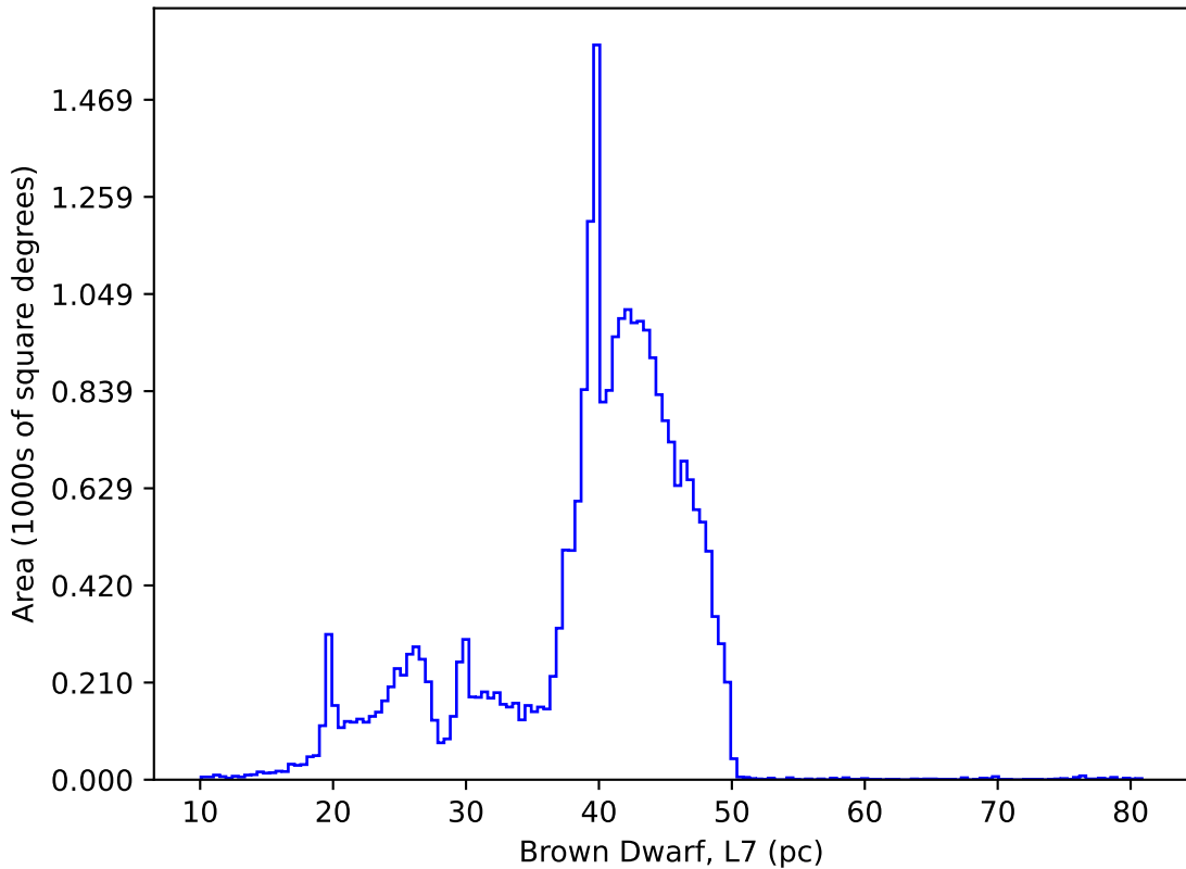
ddf_acor_sf10_lsf40_lsr50_v3.4_10yrs : Brown Dwarf, L7
