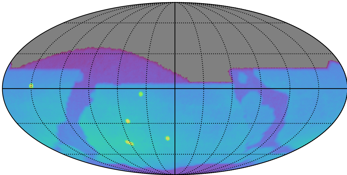
ddf_acor_sf10_lsf40_lsr50_v3.4_10yrs : Brown Dwarf, L4
