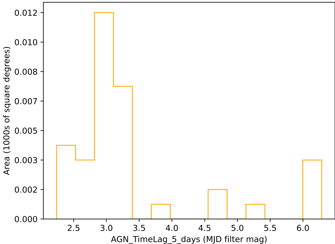
ddf_acor_sf10_lsf40_lsr50_v3.4_10yrs r band: AGN_TimeLag_5_days
