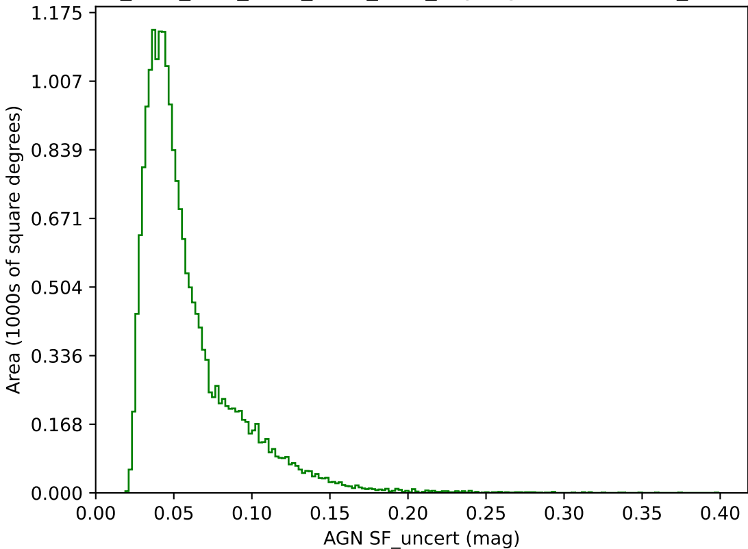
ddf_acor_sf10_lsf40_lsr50_v3.4_10yrs g band: AGN SF_uncert
