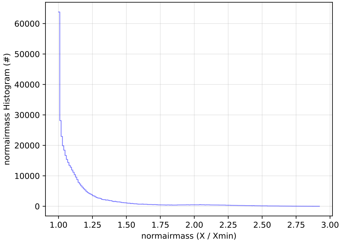
ddf_acor_sf10_lsf40_lsr50_v3.4_10yrs All sky z band: normairmass Histogram
