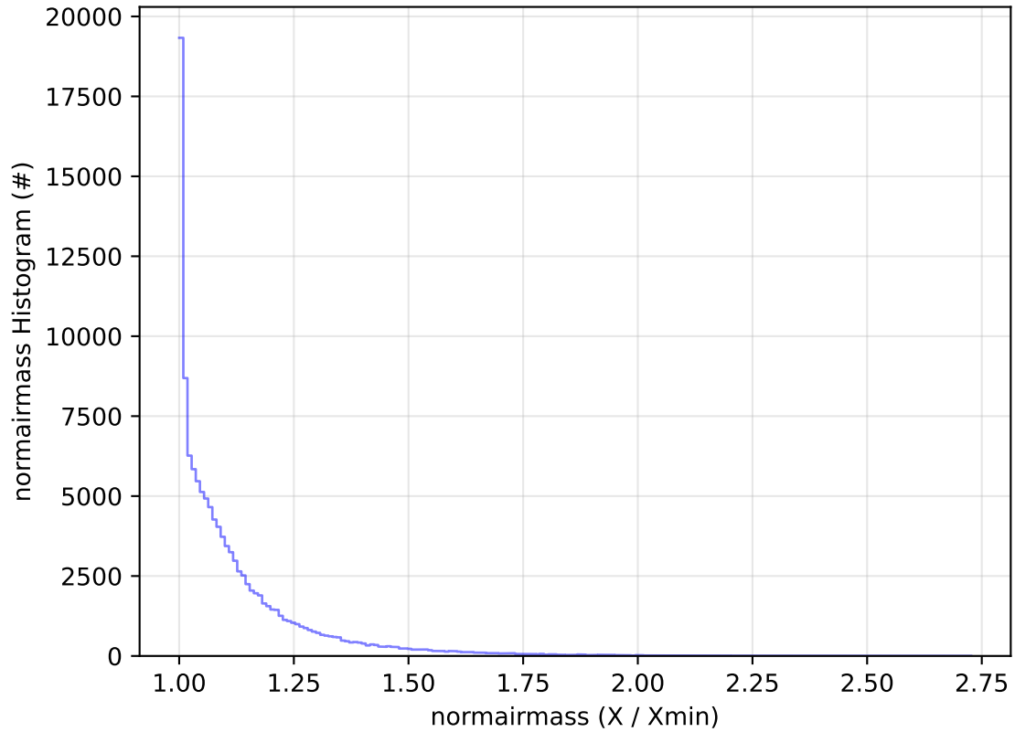
ddf_acor_sf10_lsf40_lsr50_v3.4_10yrs All sky u band: normairmass Histogram
