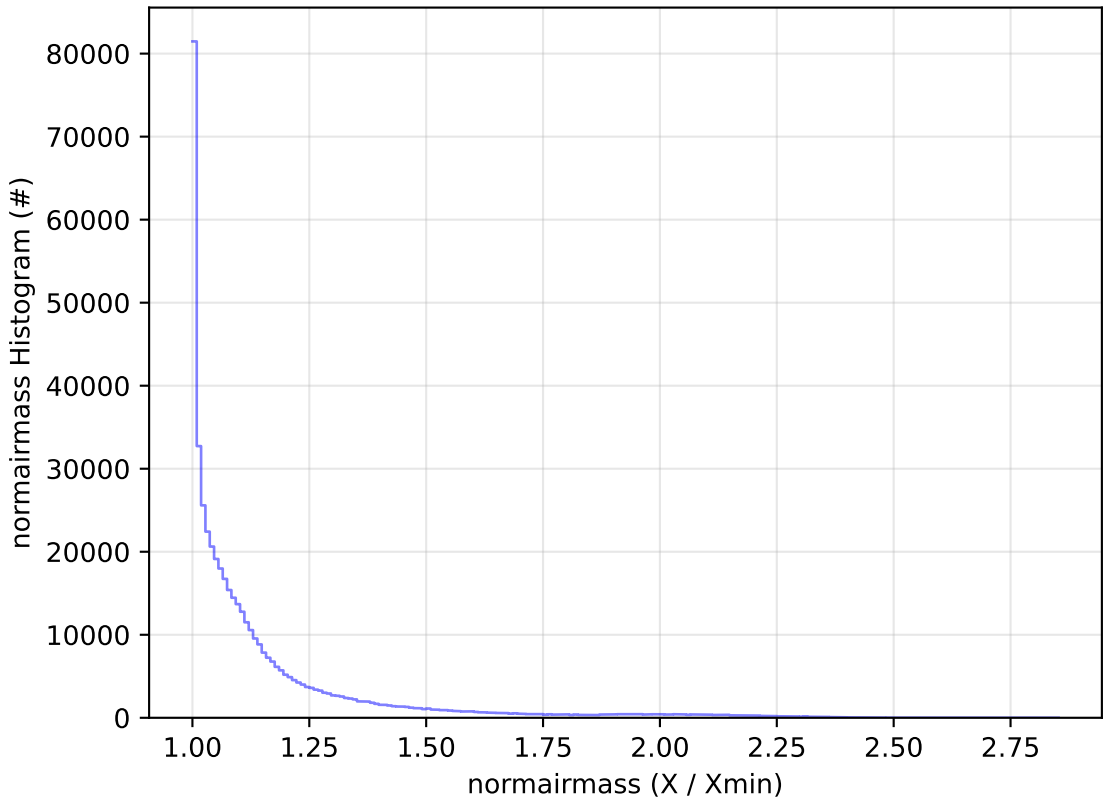
ddf_acor_sf10_lsf40_lsr50_v3.4_10yrs All sky r band: normairmass Histogram
