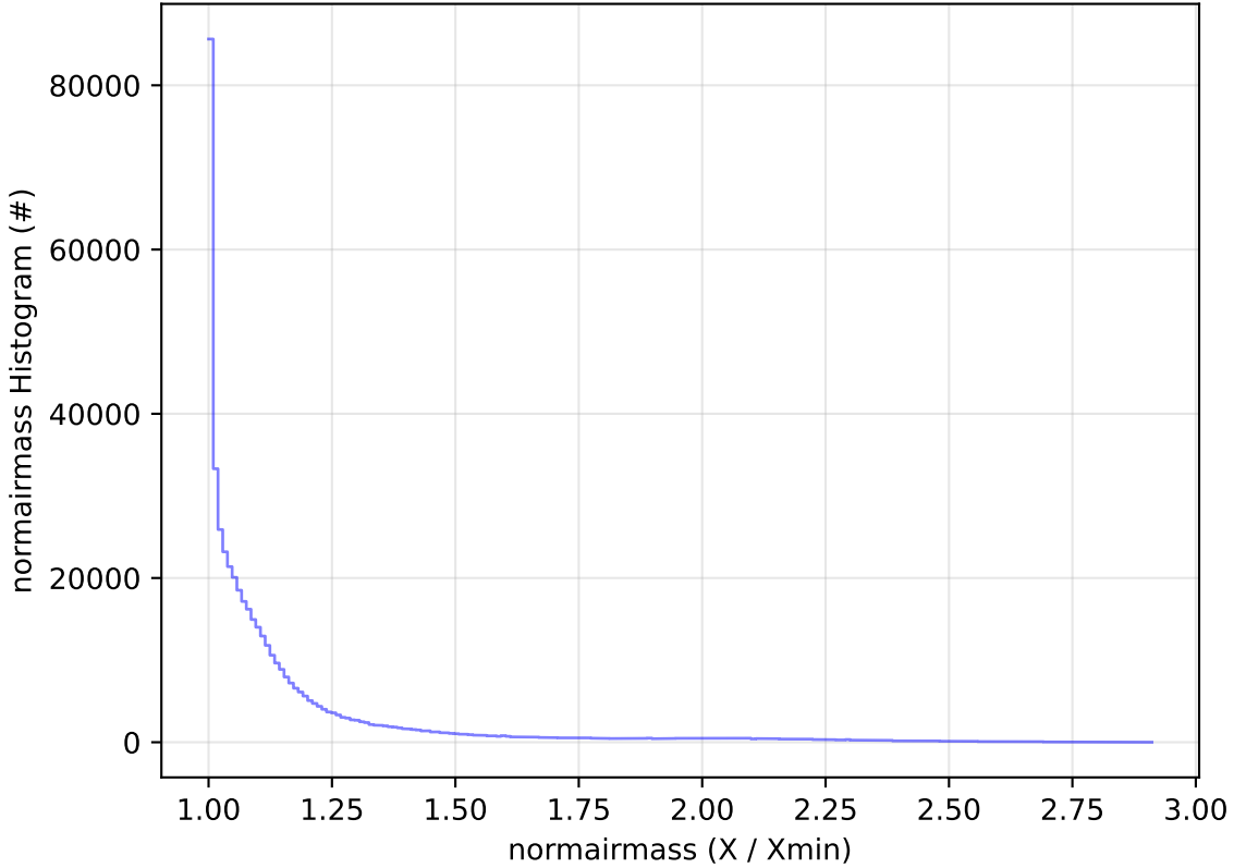
ddf_acor_sf10_lsf40_lsr50_v3.4_10yrs All sky i band: normairmass Histogram
