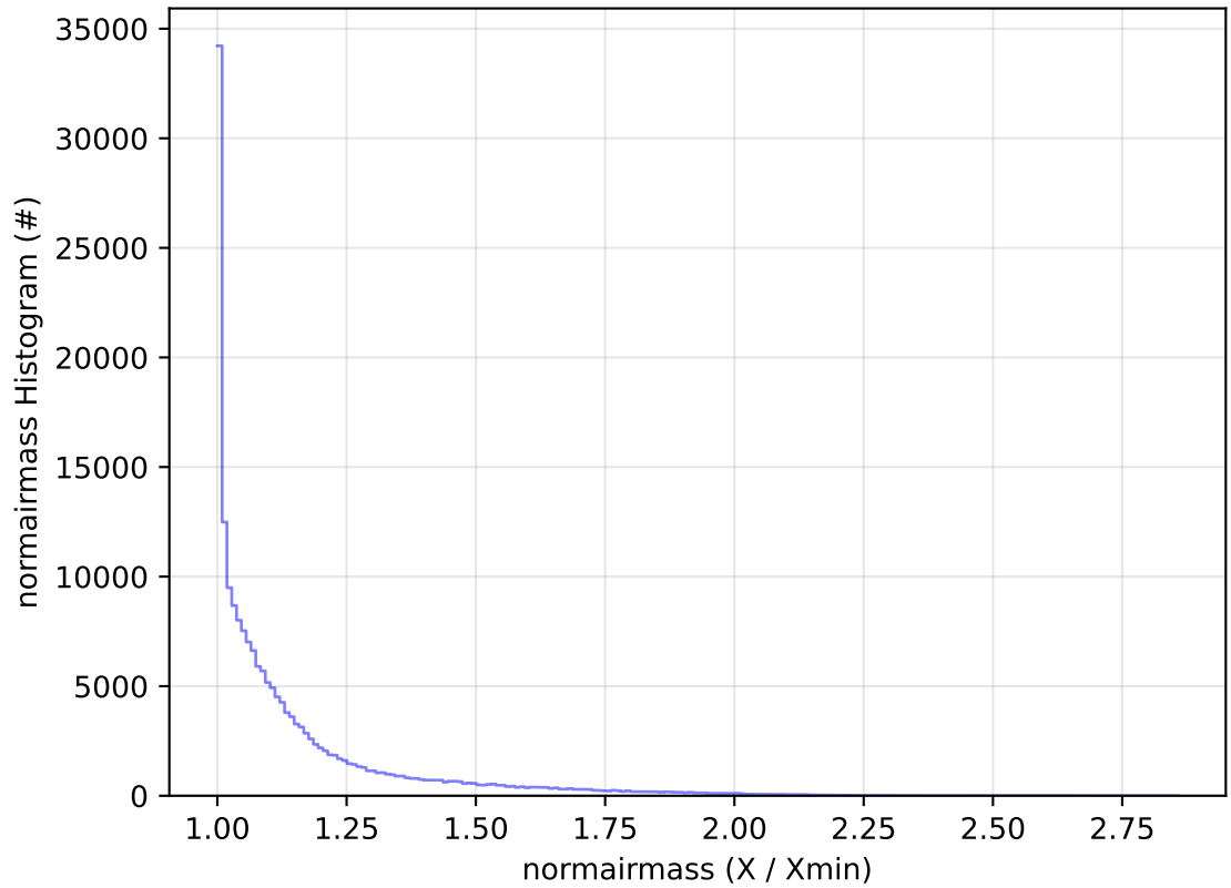
ddf_acor_sf10_lsf40_lsr50_v3.4_10yrs All sky g band: normairmass Histogram
