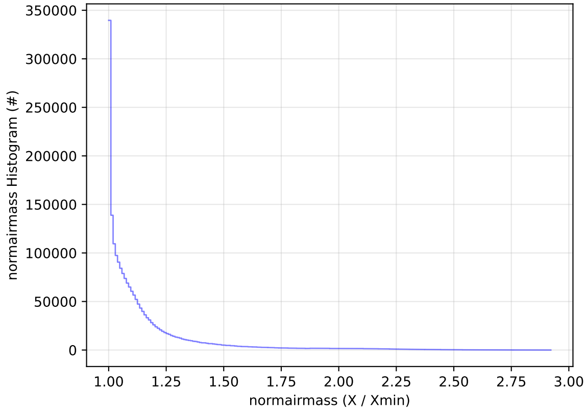
ddf_acor_sf10_lsf40_lsr50_v3.4_10yrs All sky all bands: normairmass Histogram
