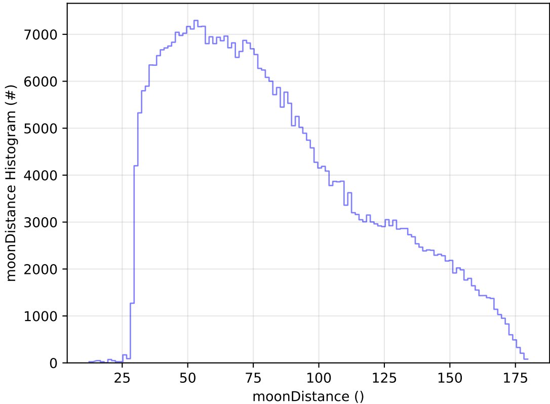
ddf_acor_sf10_ls40_lsr50_v3.4_10yrs WFD z band: moonDistance Histogram
