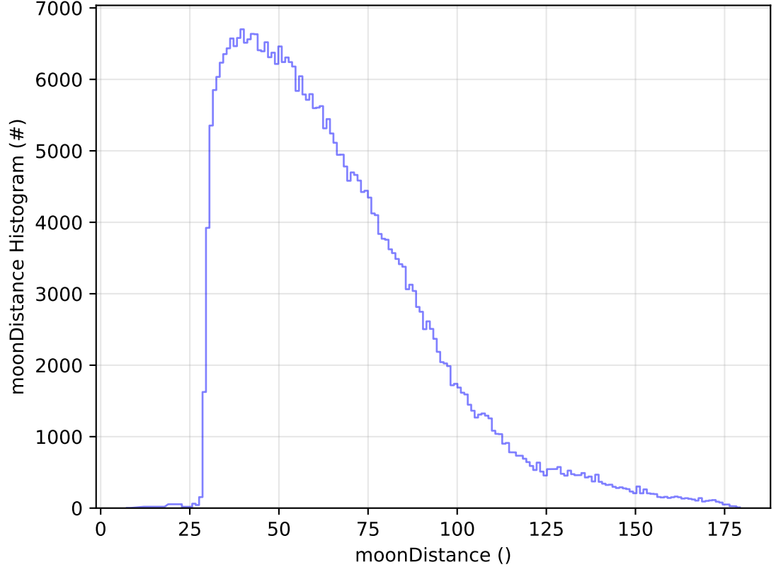
ddf_acor_sf10_Isf40_Isr50_v3.4_10yrs WFD y band: moonDistance Histogram
