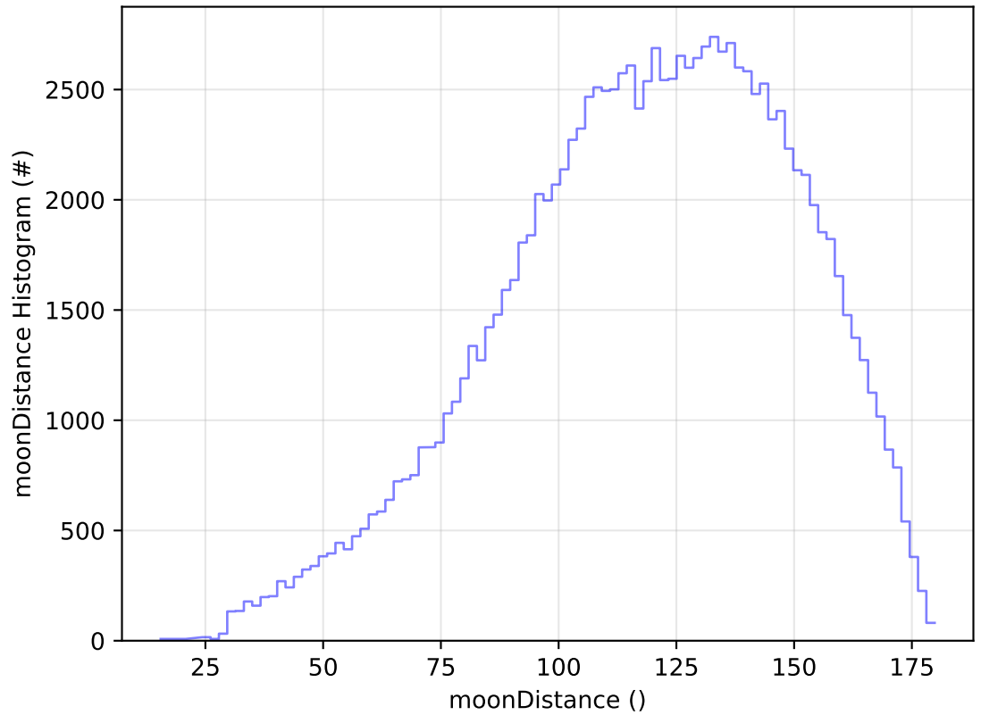
ddf_acor_sf10_lsf40_lsr50_v3.4_10yrs WFD u band: moonDistance Histogram
