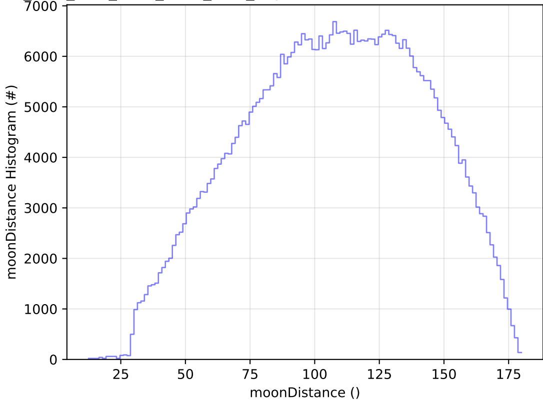
ddf_acor_sf10_lsf40_lsr50_v3.4_10yrs WFD r band: moonDistance Histogram
