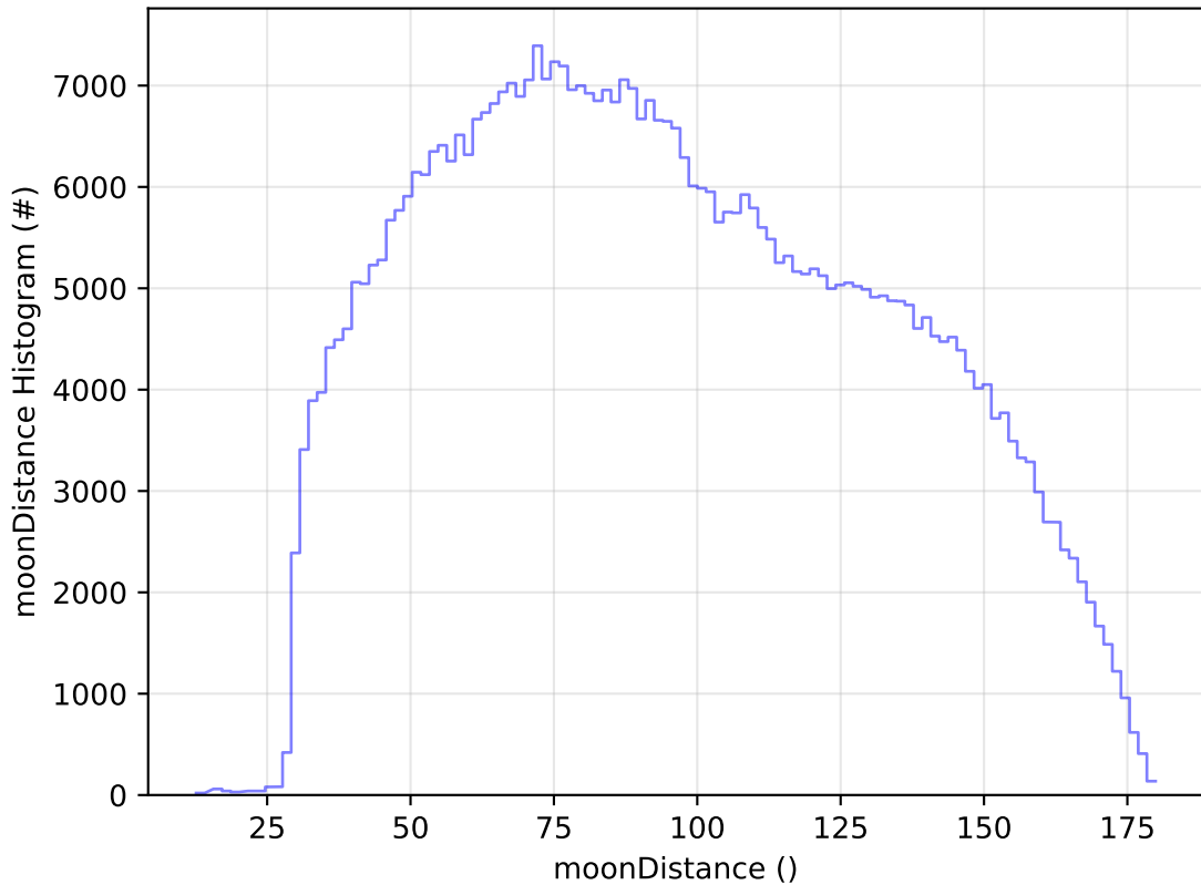
ddf_acor_sf10_lsf40_lsr50_v3.4_10yrs WFD i band: moonDistance Histogram
