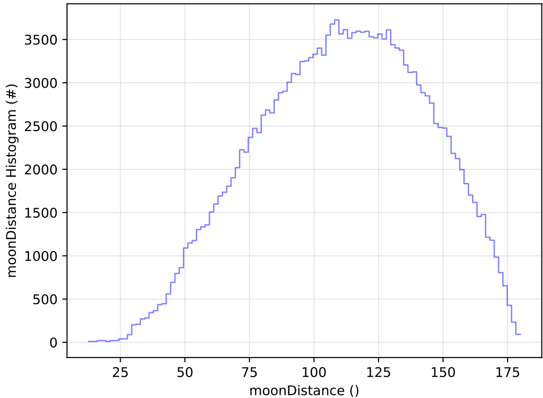
ddf_acor_sf10_lsf40_lsr50_v3.4_10yrs WFD g band: moonDistance Histogram
