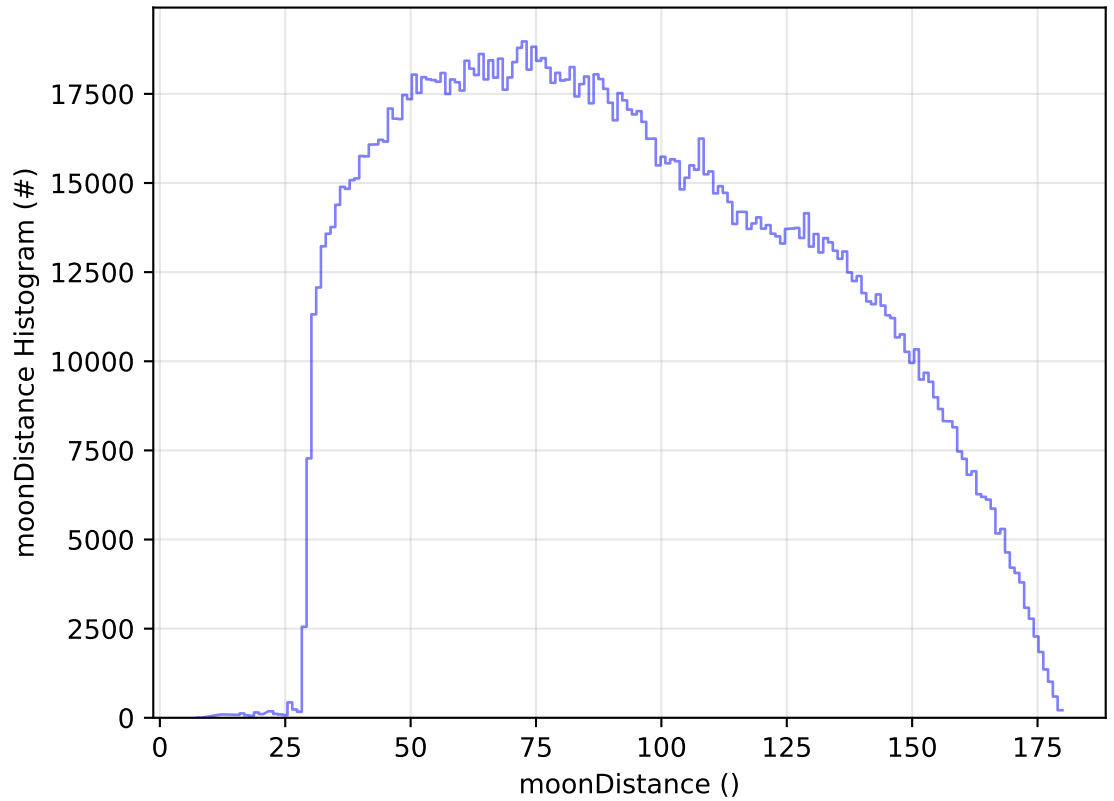
ddf_acor_sf10_lsf40_lsr50_v3.4_10yrs WFD all bands: moonDistance Histogram
