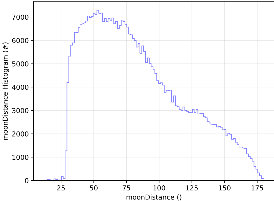
ddf_acor_sf10_lsf40_lsr50_v3.4_10yrs All sky z band: moonDistance Histogram
