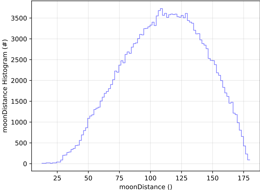
ddf_acor_sf10_lsf40_lsr50_v3.4_10yrs All sky g band: moonDistance Histogram
